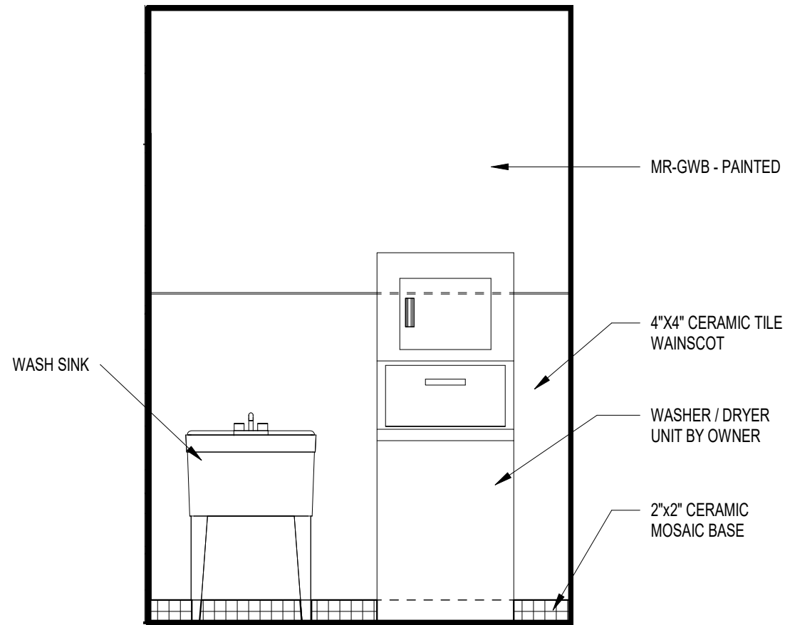
① LAUNDRY - WEST- AMENDED PERMIT 1/2" = 1'-0"
